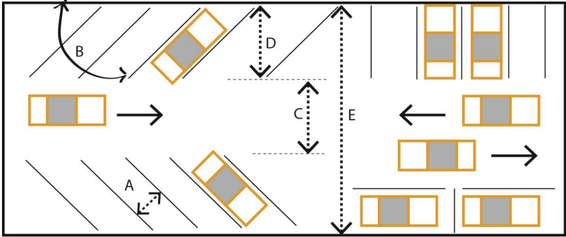
Figure 23. Parking Diagram
